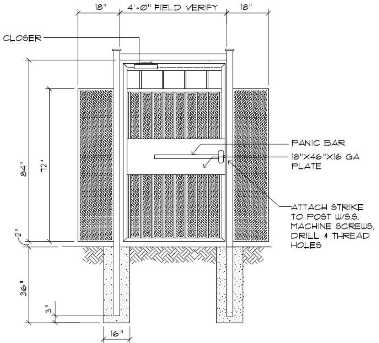
Typical Gate G1 DETAIL
